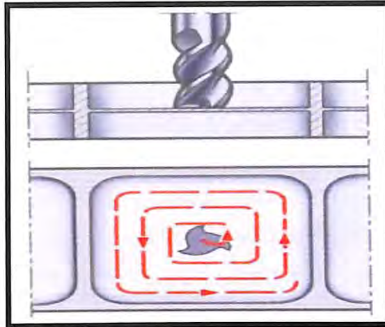
Figure 2.4: Strategy for the milling of thin-bases (Smith, 2008)
