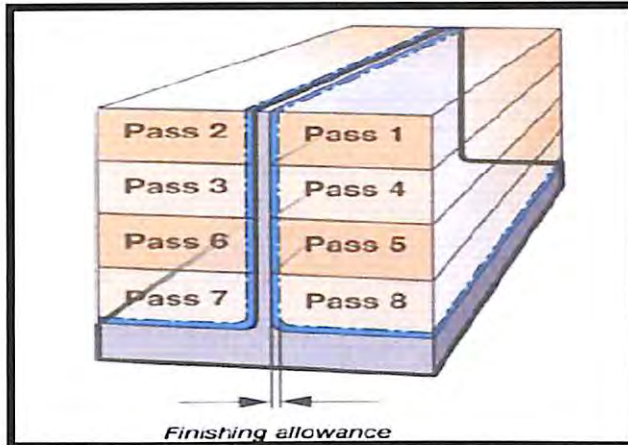
Figure 2.1: Waterline milling (Smith, 2008)
