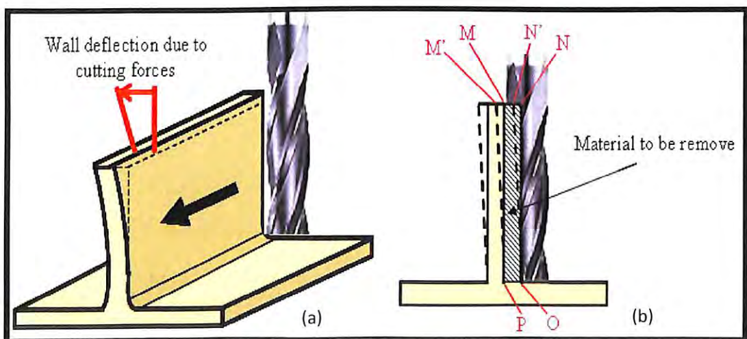
Figure 1.2: Dimensional surface errors produce in machining thin-wall feature
