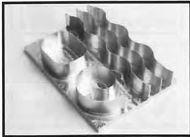
Figure 2.3: Unsupported thin-base features (Smith, 2008)
