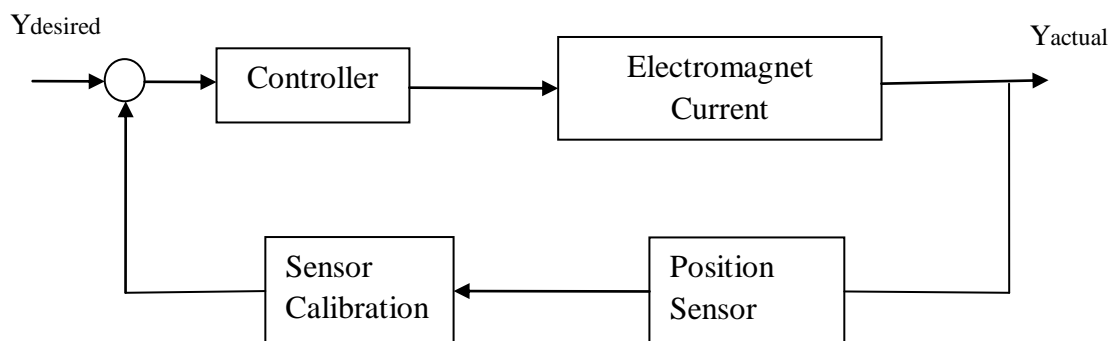
Figure 2.1: Basic Schematic System of MagLev
