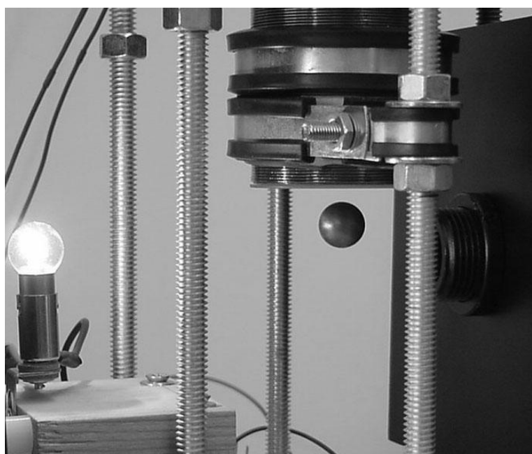
Figure 2.8: Stable Levitation of Steel Ball
