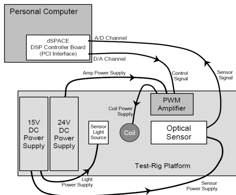
Figure 2.6: Magnetic Levitation System Schematic Diagram
